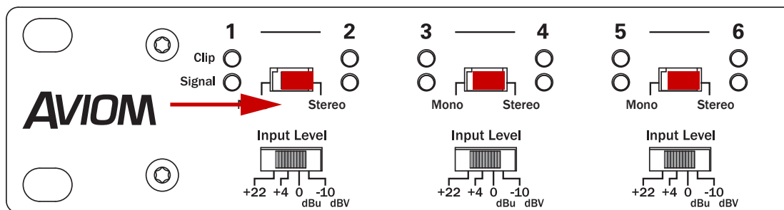
Stereo Links on the AN-16/i Input Module
