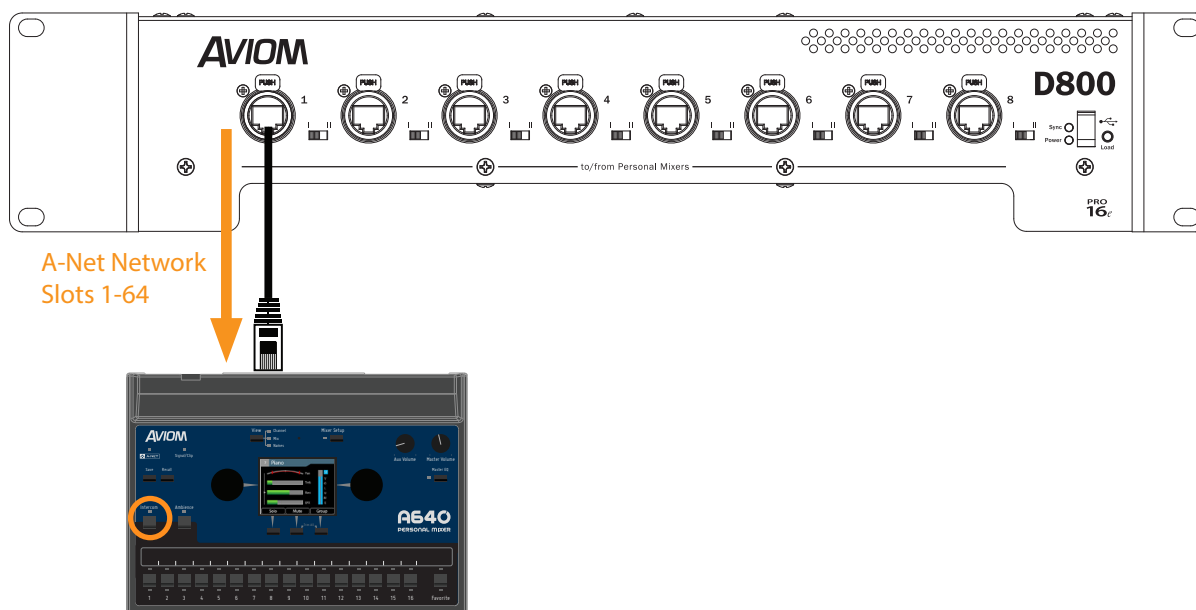
64 network channels are sent to an A640 from a D800.
