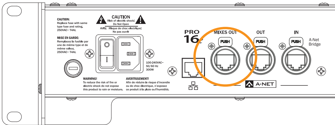
The Mixes Out port on the D800
