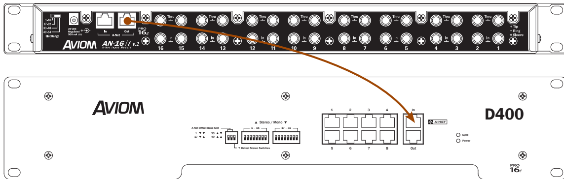
A-NET OUT on the analog input device is connected to A-NET IN on the D400.
