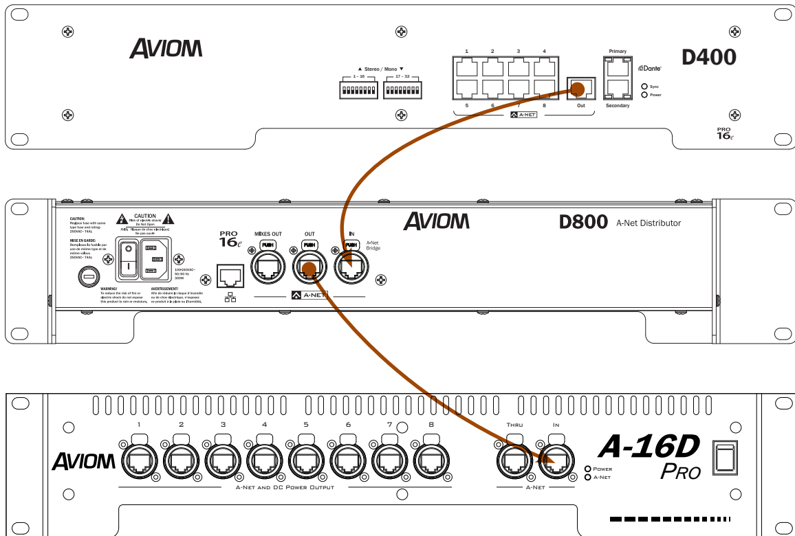
An expanded network using a D400, D800, and A-16D Pro allows up to 24 Personal Mixers to be connected.
