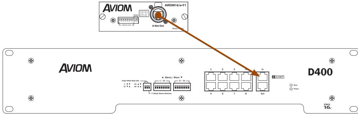
A-NET OUT from the console card is connected to A-NET IN on the D400.
